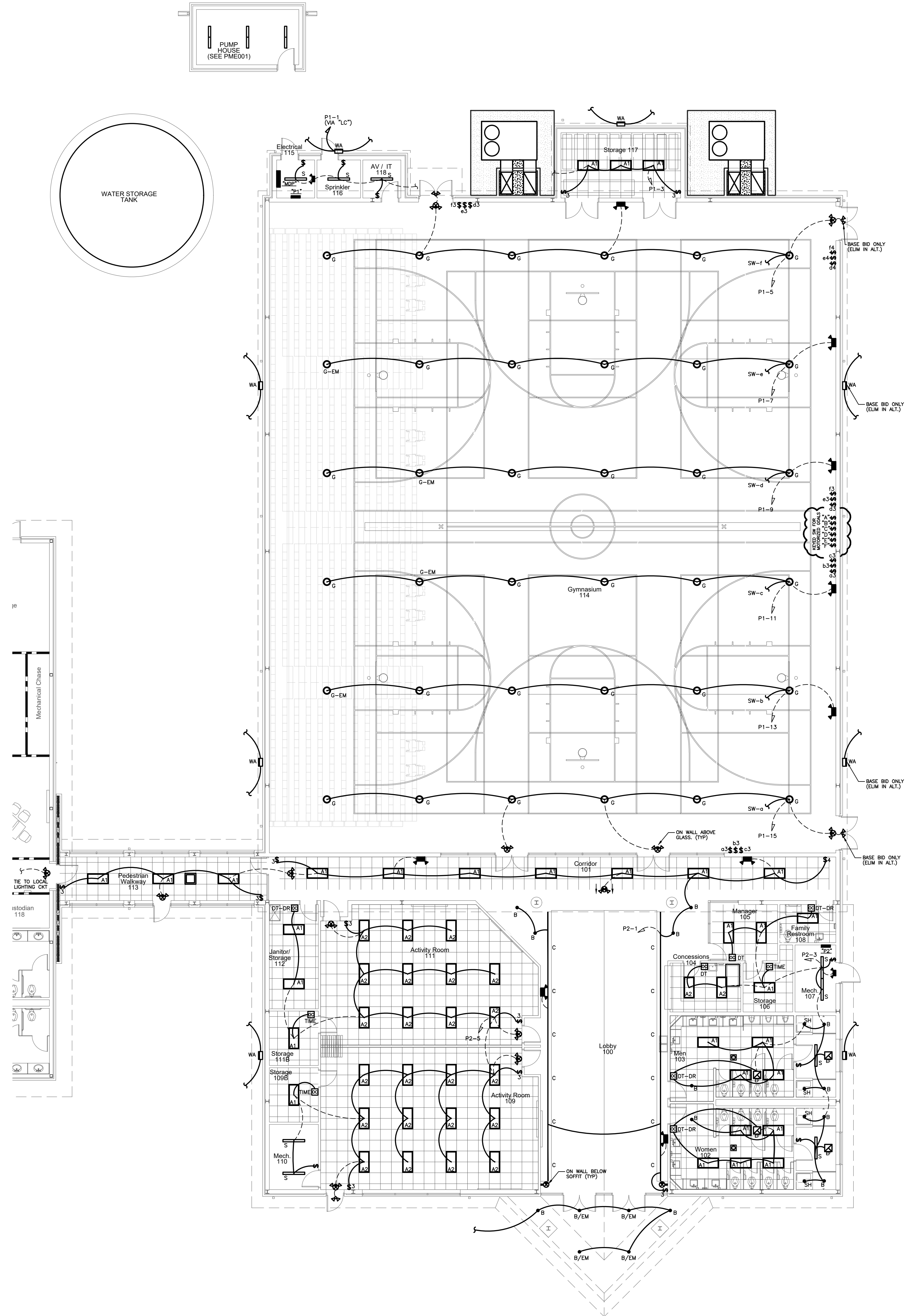
LIGHTING PLAN (BASE BID)
