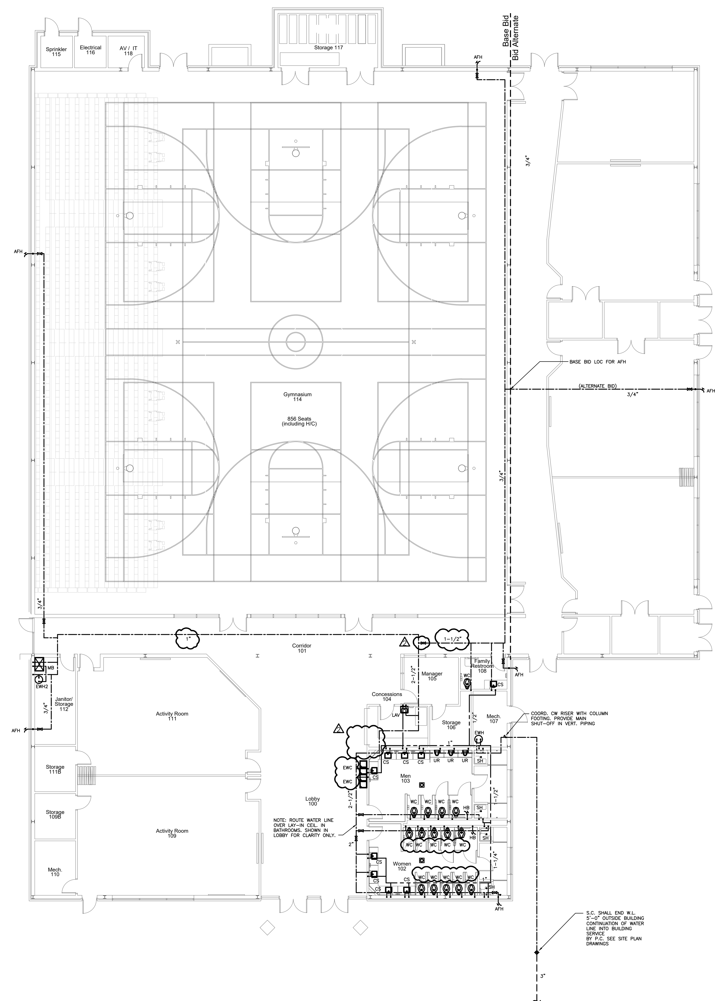
DOMESTIC WATER PLAN SCALE: 3/32" = 1'-0"
