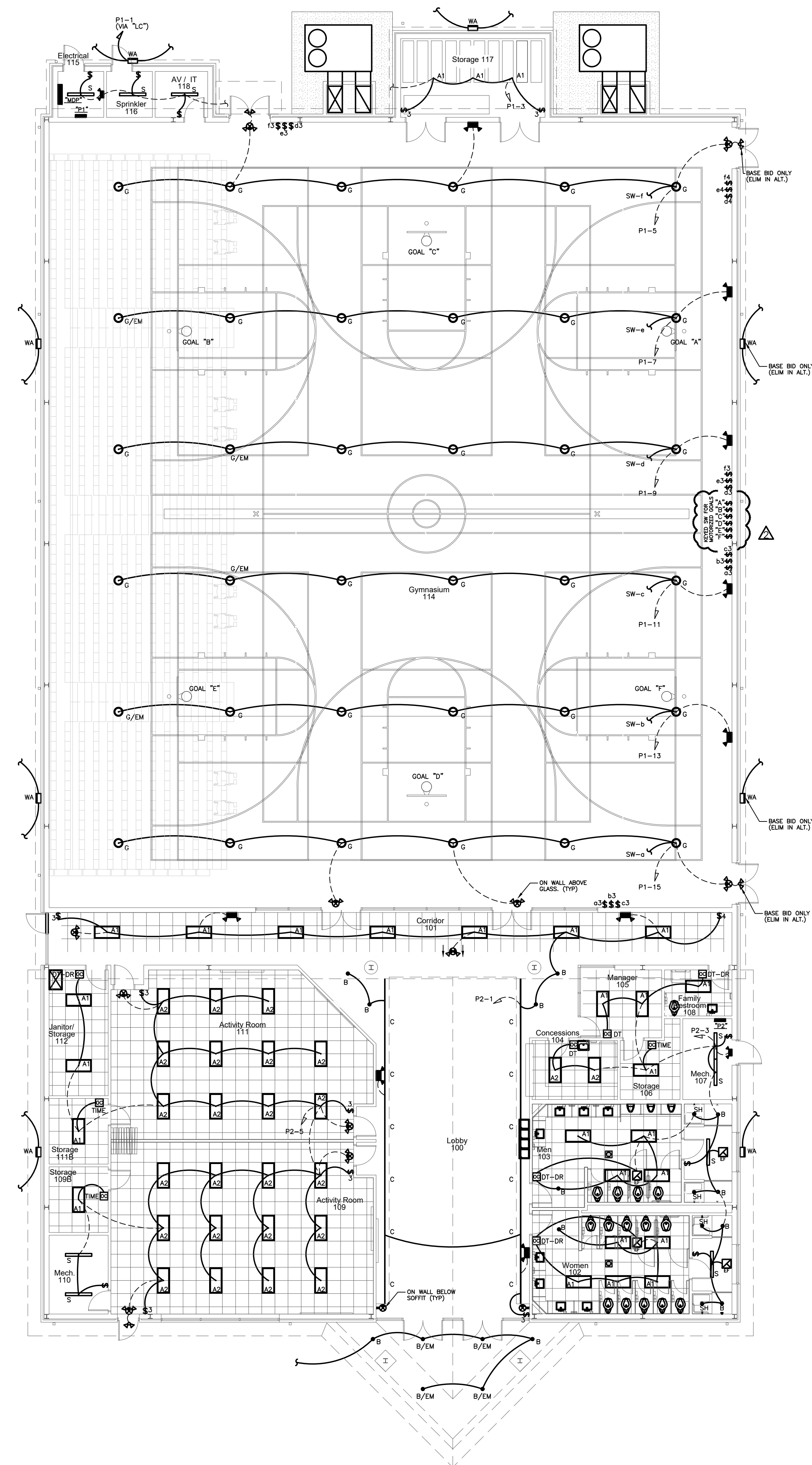
LIGHTING PLAN (BASE BID) SCALE: 3/32" = 1'-0"
