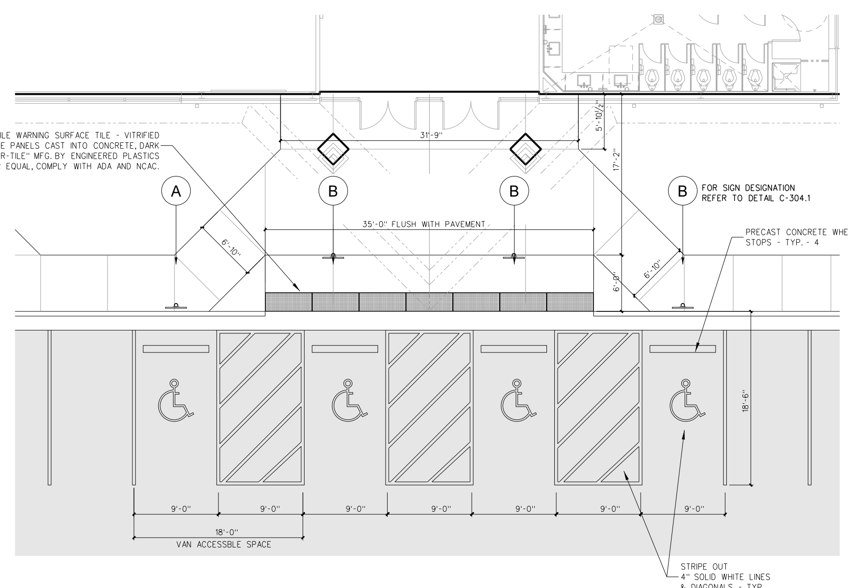
101.2 ACCESSIBLE PARKING SPACES
