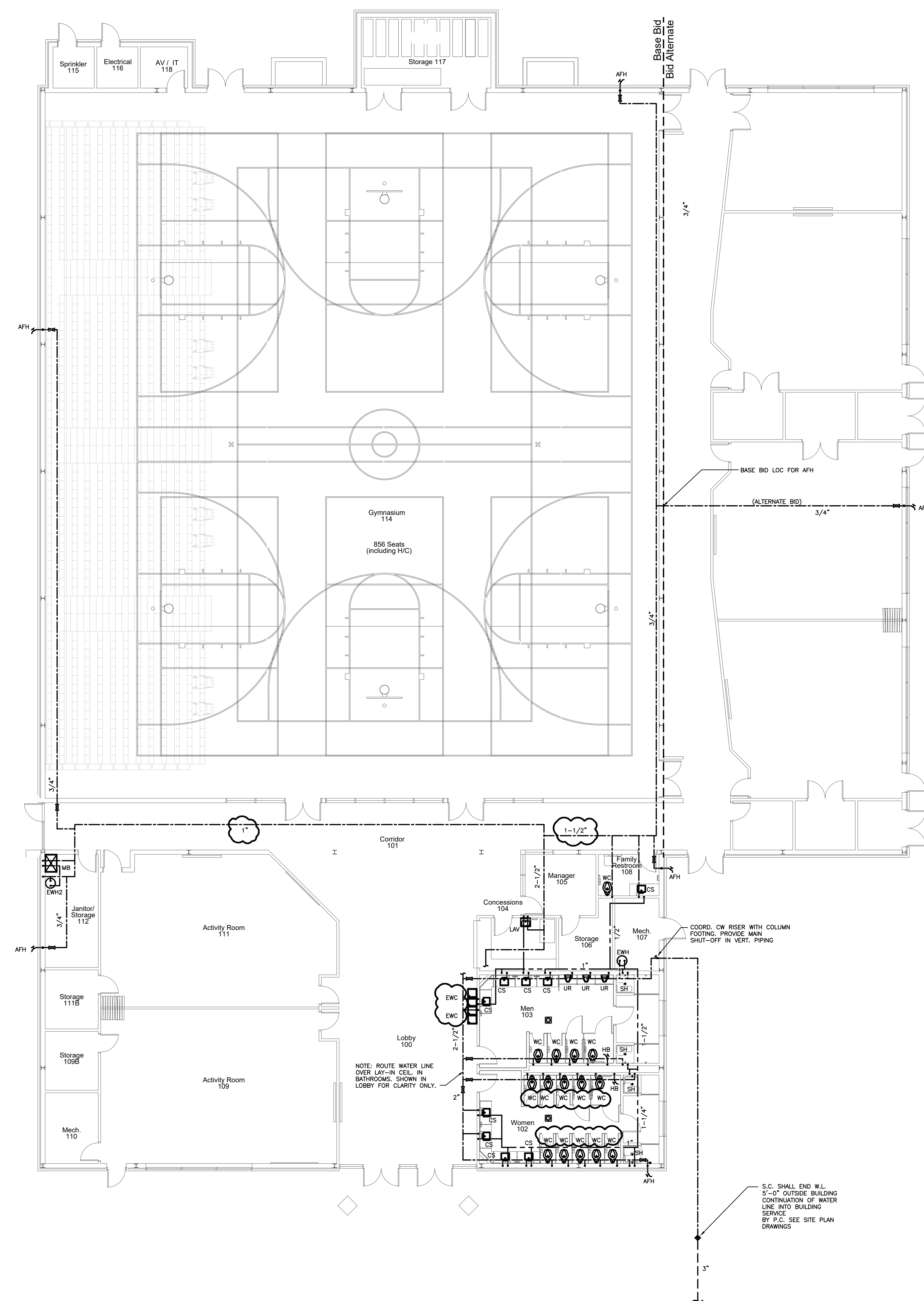
DOMESTIC WATER PLAN SCALE: 3/32" = 1'-0"
