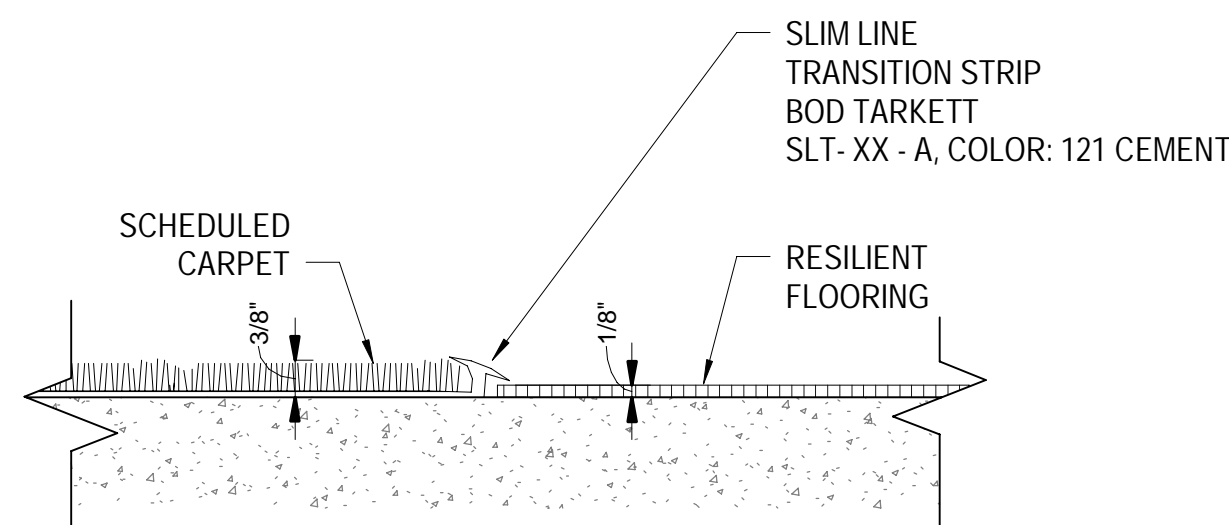
TS - 1 CARPET TO RESILIENT
