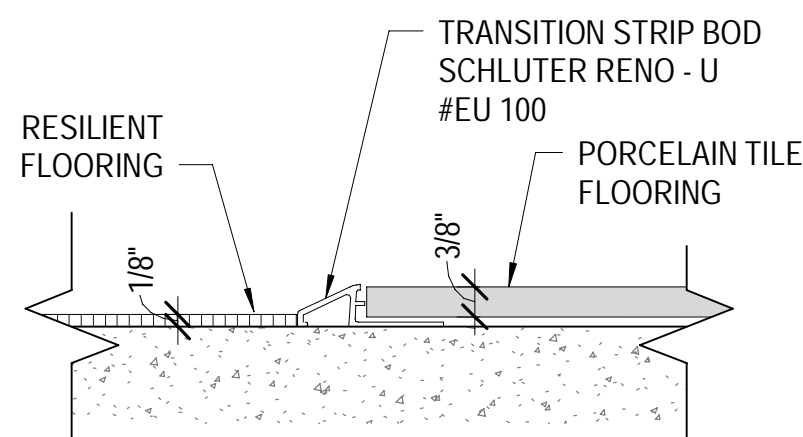
TS - 3 RESILIENT TO PORCELAIN
