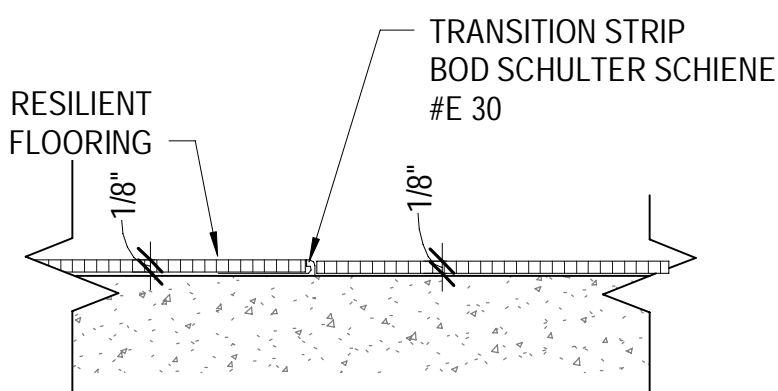
TS - 4 RESILIENT TO STATIC DISSIPATIVE TILE
