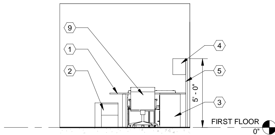
F4 DL-01 PRIVATE OFFICE TYPICAL - WEST ELEVATION 1/4" = 1'-0"
