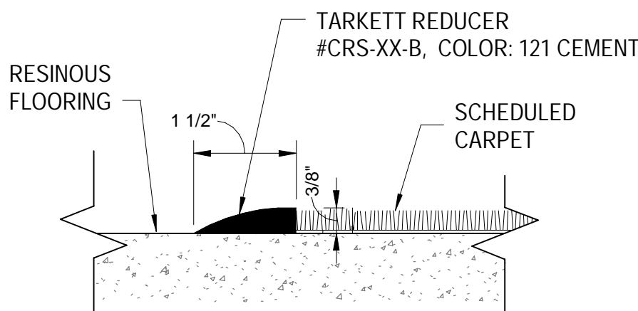
TS - 5 CONCRETE TO CARPET
