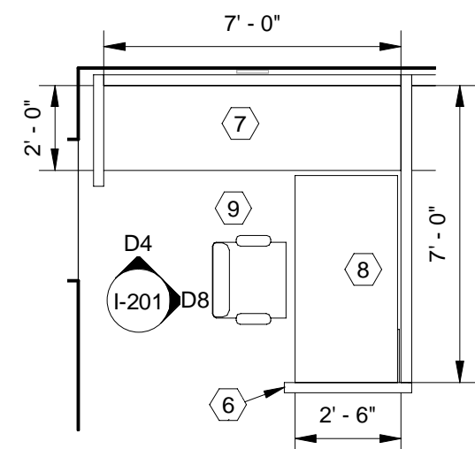
(D1) WS-01 WORKSTATION TYPICAL - PLAN VIEW 1/4" = 1'-0"
