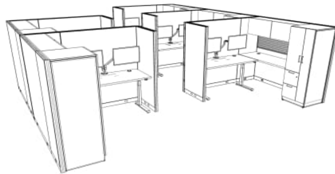
(B4) WS-01 WORKSTATION ISOMETRIC VIEW 3" = 1'-0"
