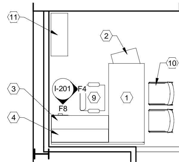
F1 DL-01 PRIVATE OFFICE TYPICAL - PLAN VIEW 1/4" = 1'-0"
