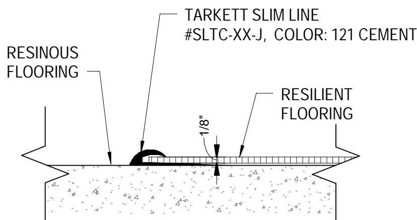
TS - 2 CONCRETE TO RESILIENT
