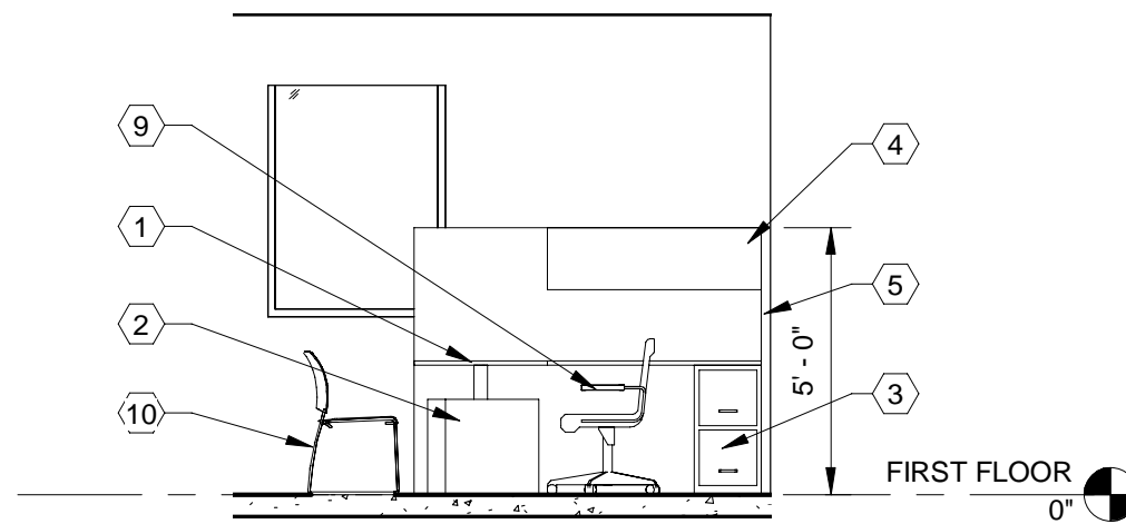
F8 DL-01 PRIVATE OFFICE TYPICAL - NORTH ELEVATION 1/4" = 1'-0"
