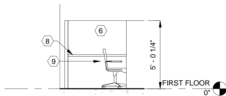
D4 WS-01 WORKSTATION TYPICAL - NORTH ELEVATION 1/4" = 1'-0"
